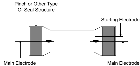
Figure 1 ARC TUBE
